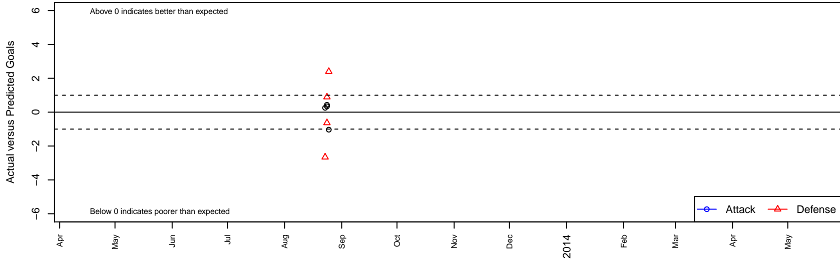
Flames United FC B02 Dots are actual minus expected GF (blue circles) and GA (red triangles). Blue line is smoothed change in attack strength. Red is smoothed change in defense strength.
